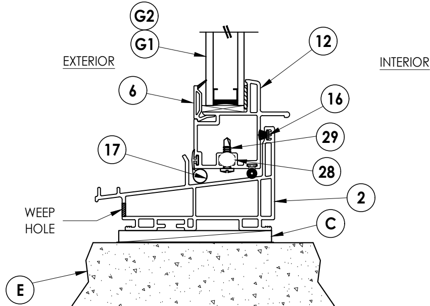
3 VERTICAL CROSS SECTION 3 Shown direct to masonry
