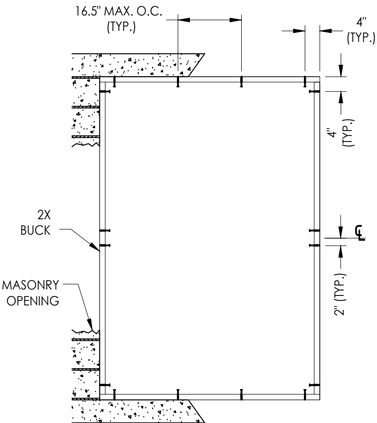
BUCK ANCHORING
